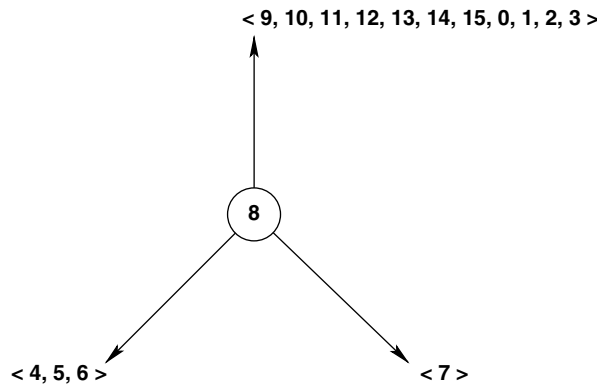
FIGURE 4.19: Disjoint intervals
