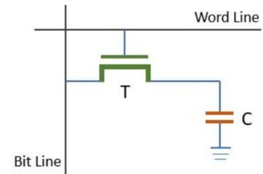
Single Transistor Dynamic Memory Cell
