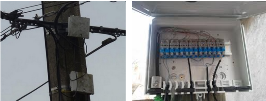
Figure II.4. Point de concentration (PC)
